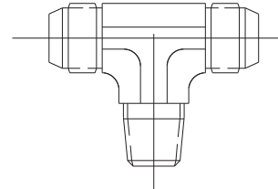
MALE BRANCH TEE 1/8" NPT x 5/15" TUBING P/N WK-699205-050
