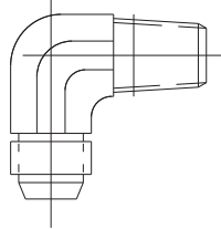
MALE ELBOW 1/8" NPT x 5/16" TUBING P/N WK-699205-030
